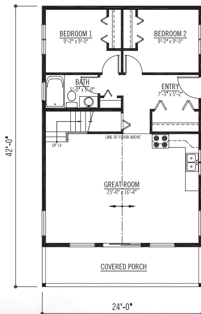
MAIN FLOOR
