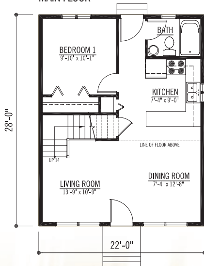
MAIN FLOOR
