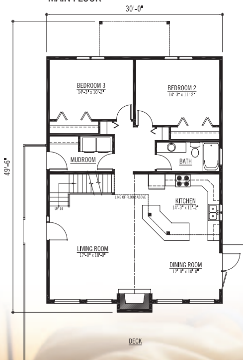
MAIN FLOOR
